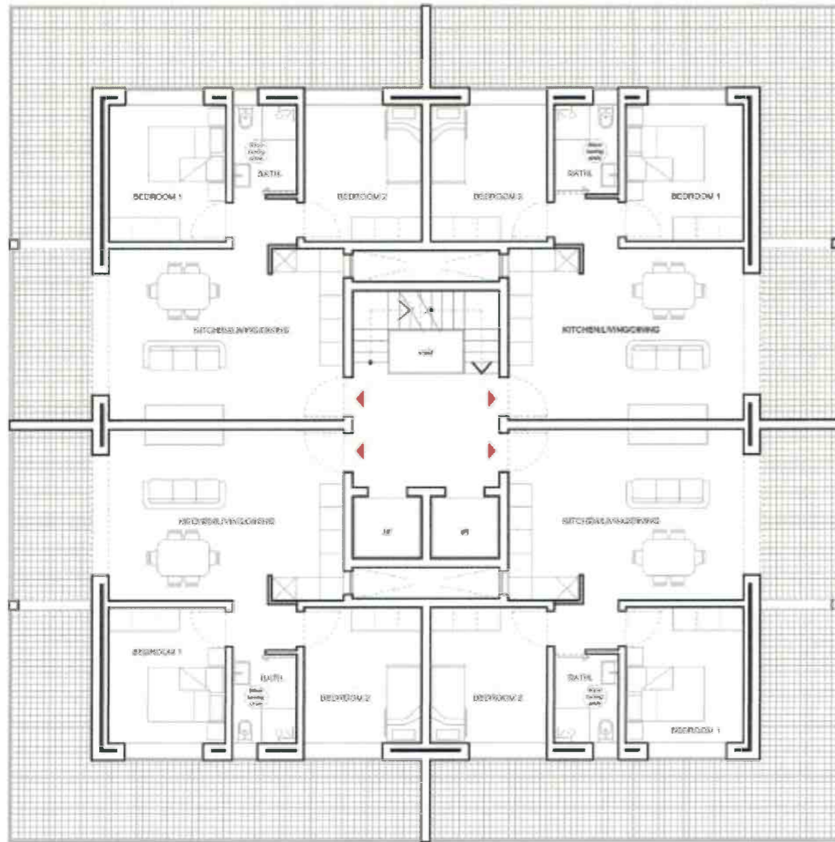
Typical Floor Furniture Layout Scale: 1:100
