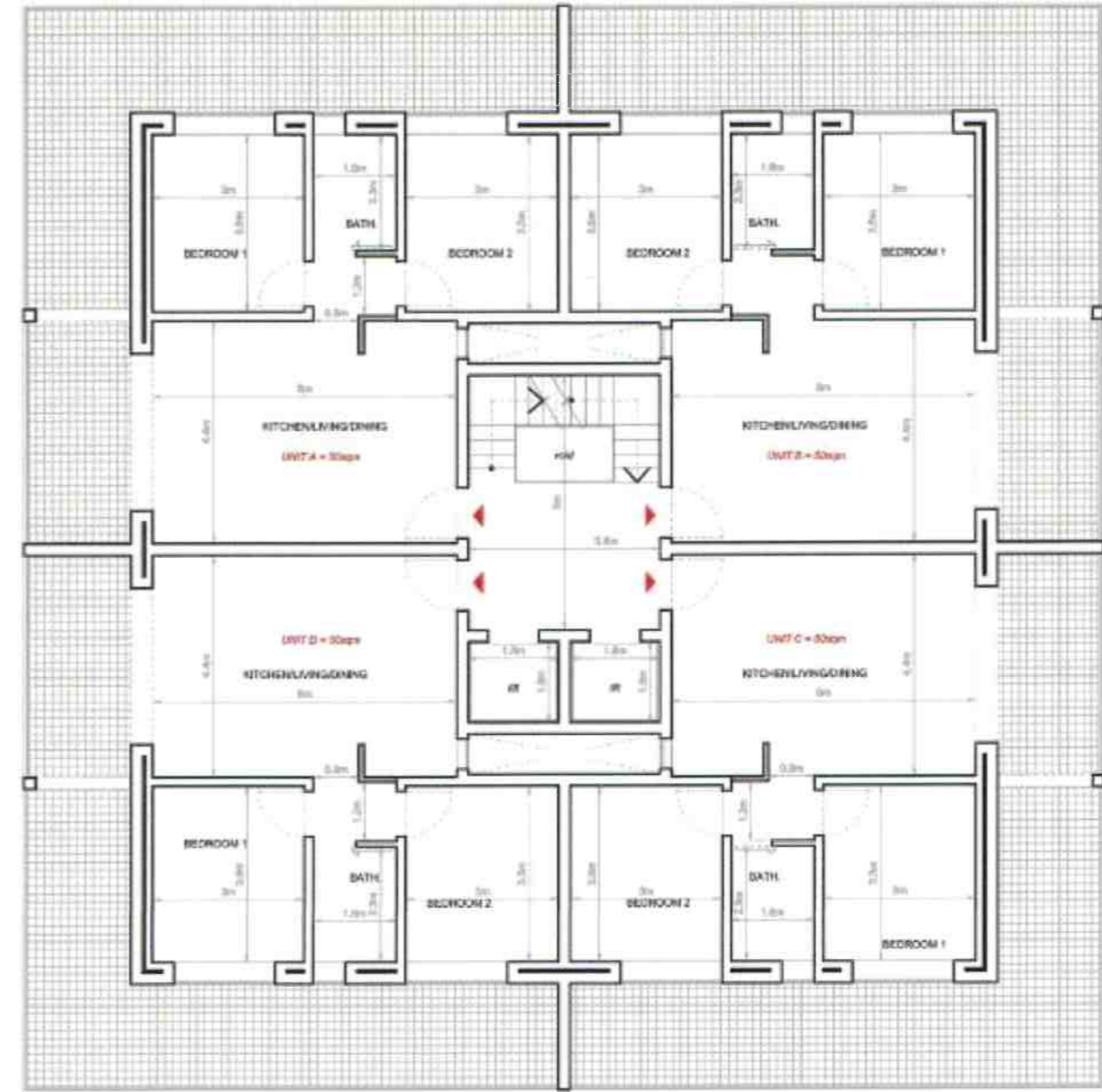
Typical Floor Dimension Layout Scale: 1:100
